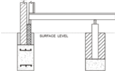
Fig. 3 Strip & Stump Footing System
